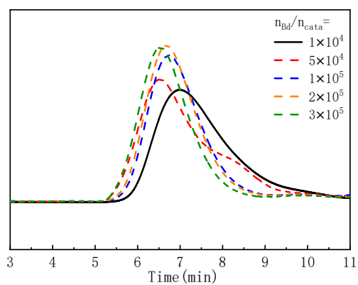
Fig.S1 The GPC curves of HVBR-g-COOH prepared by metathesis catalyst with different addition loadings
