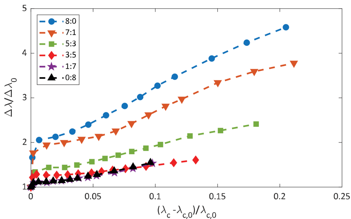
Fig. S1 Change in the normalized reflection bandwidth versus the normalized reflection notch center for samples prepared with 8wt% monomer, 5wt% S1011, 5wt% S811, 1wt% I-369 in MLC-2079. The weight ratio of RM82: HDDA was changed between each sample as indicated in the legends. Polymerization was initiated by UV light (365nm, 50 mW/cm 2 ) for 10 min.
