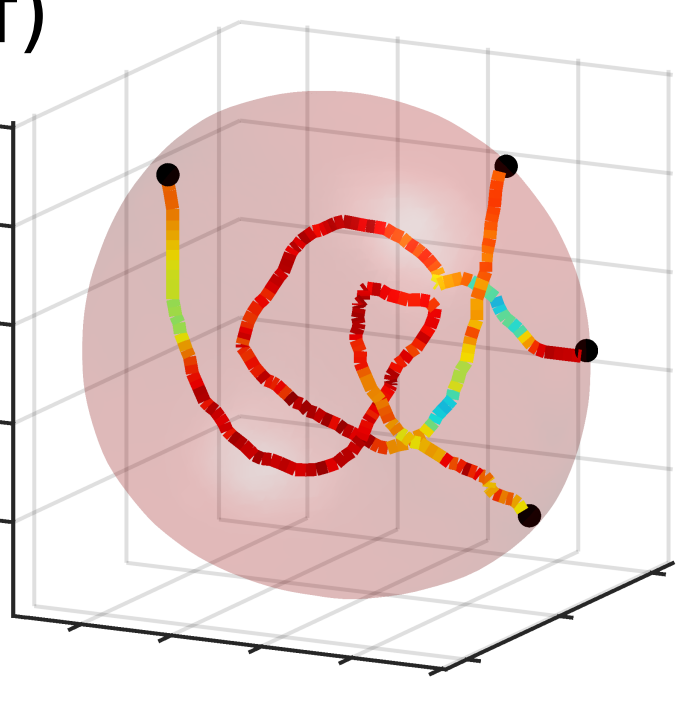
Active turbulence
