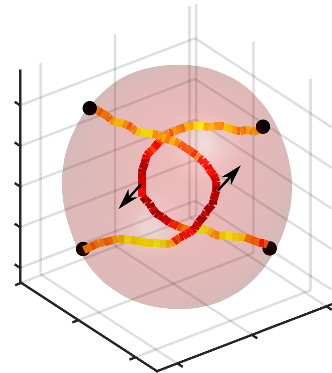
Disclination dance
