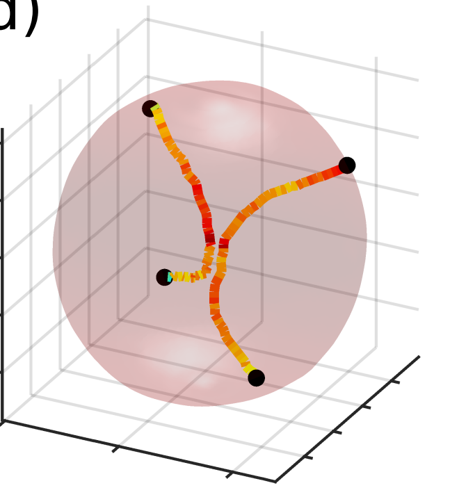
Stable +1 defect
