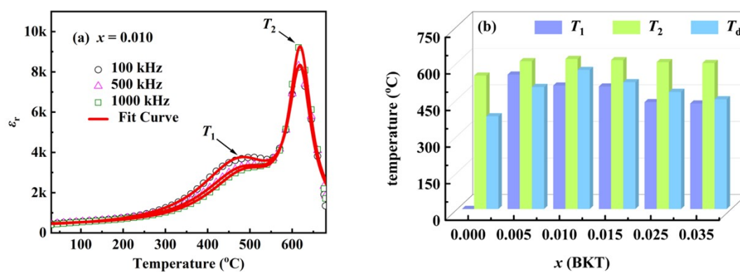
Fig. S1 (a) Temperature dependence of dielectric permittivity ( \epsilon_r ) for BF-BT-0.010BKT ceramics as a function of frequency; (b) variations of phase transition temperatures ( T_2 ), Dielectric anomaly ( T_1 ) and T_d for the BF-BT- x BKT.
