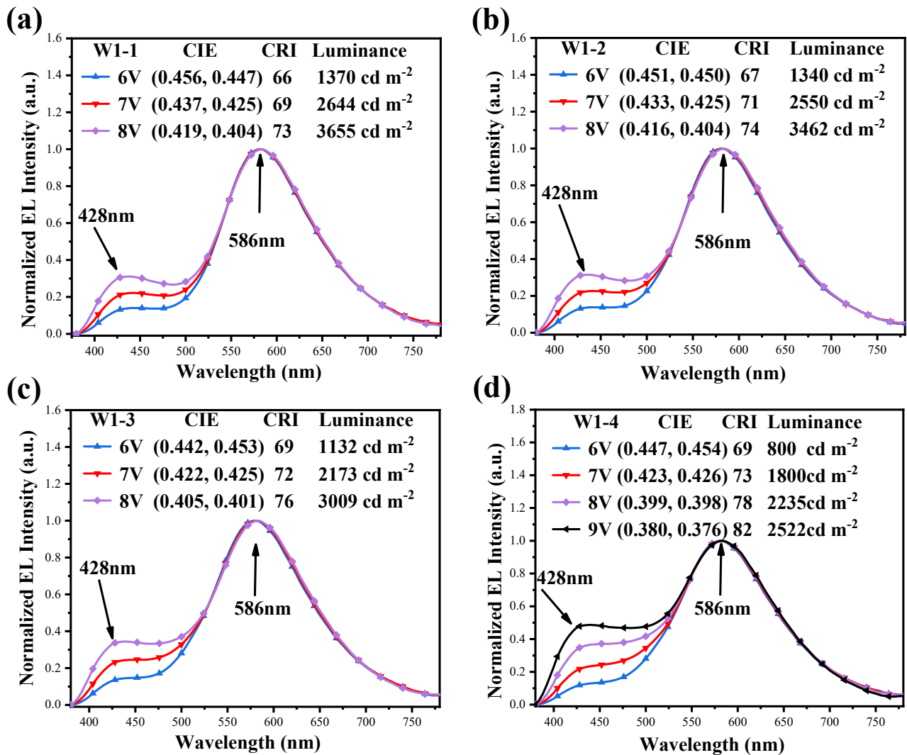
Fig. S1 Normalized EL spectra for white devices W_{1-1} to W_{1-3} at a driving voltage range of 6-8V and for device W_{1-4} at a driving voltage range of 6- 9 V.
