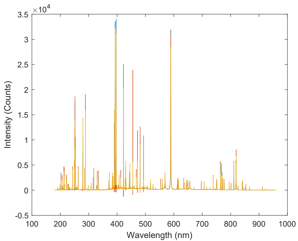
SI 2 Raw LIBS spectra of three differently colored red glasses used in this study.
