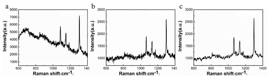
Figure. S3 The optimization results of the PE Raman spectra (a) original spectrum, (b) baseline-subtracted spectrum, and (c) smoothed spectrum
