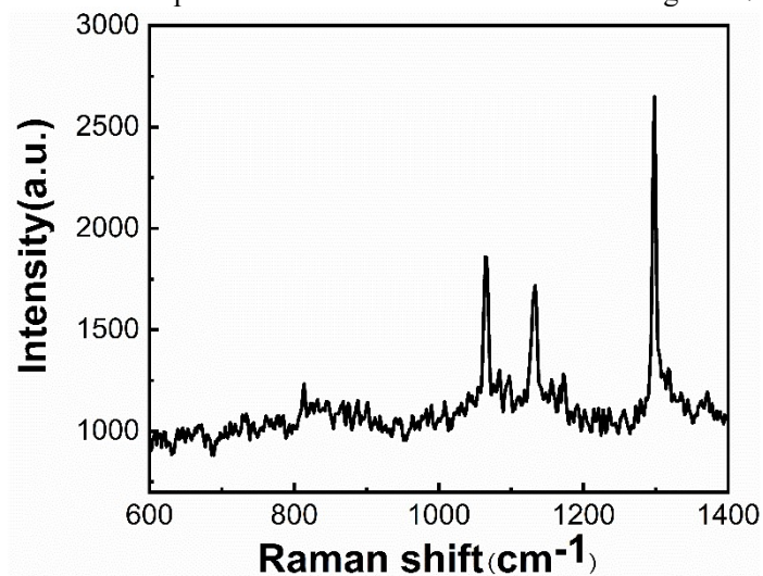
Figure. S2 Raman spectrum of PE under excitation wavelength of 532 nm
