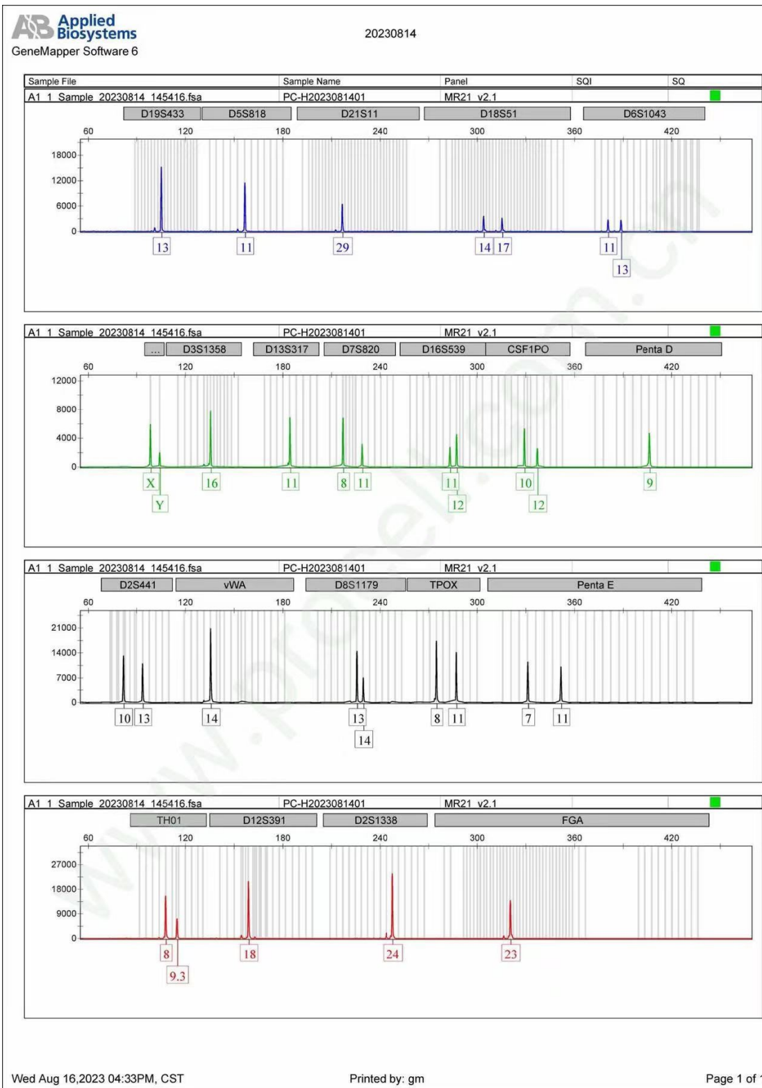
Figure 1: STR identification of A549 cell
