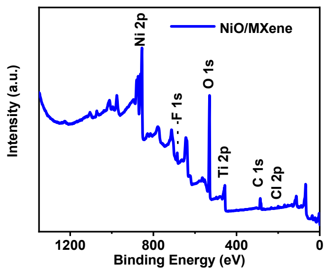
Fig. S1 The full XPS spectrum of NiO/Ti 3 C 2 T x .
