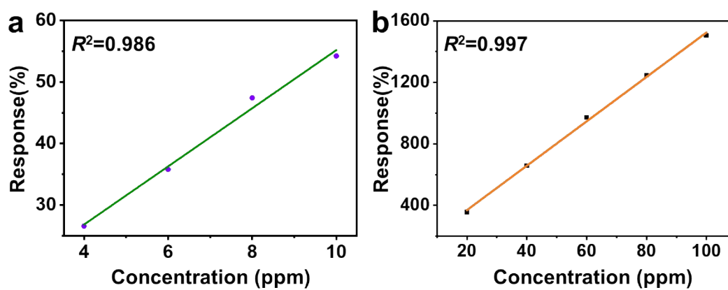
Fig. S2 The fitting curves between gas concentrations and response values of the NiO/Ti 3 C 2 T x sensor.
