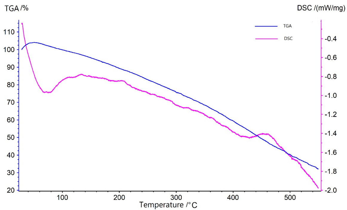
Fig. S2 TGA and DSC of the boehmite
