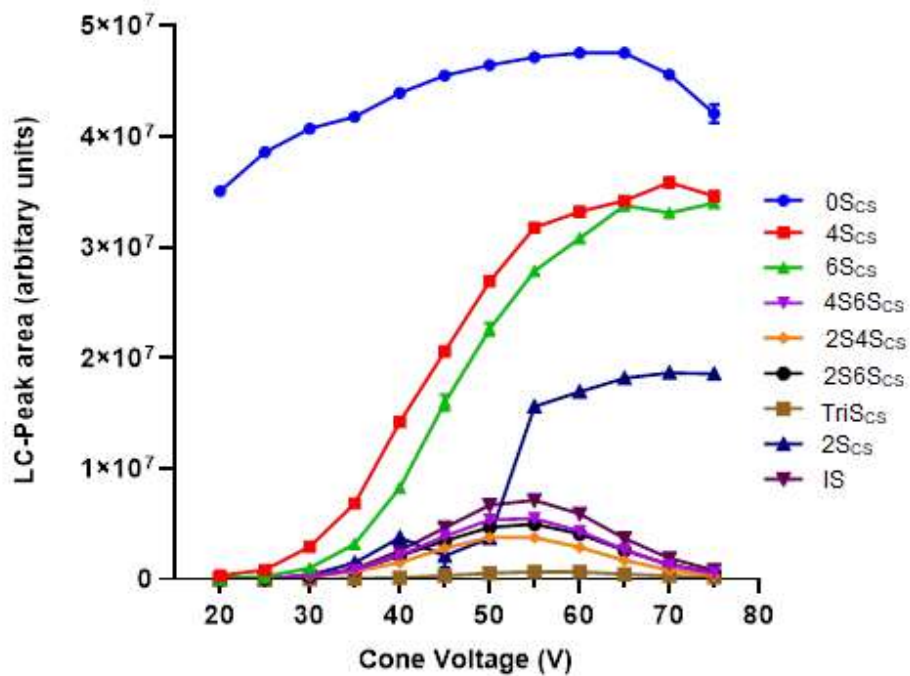
Figure S-3: LC-Peak area of procainamide-derivatised CS disaccharides and disaccharide internal disaccharide standard (20 µg/mL each) as a function of MS cone voltage.
