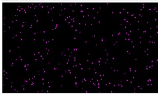
S K \alpha 1
