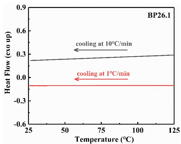
Figure S3. DSC cooling curves at 10 °C/min and 1 °C/min of BP26.1.
