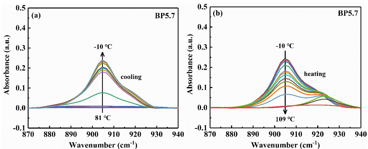
Figure S2. In-situ FTIR spectra of BP5.7 during (a) cooling (b) heating process with 10 °C/min.
