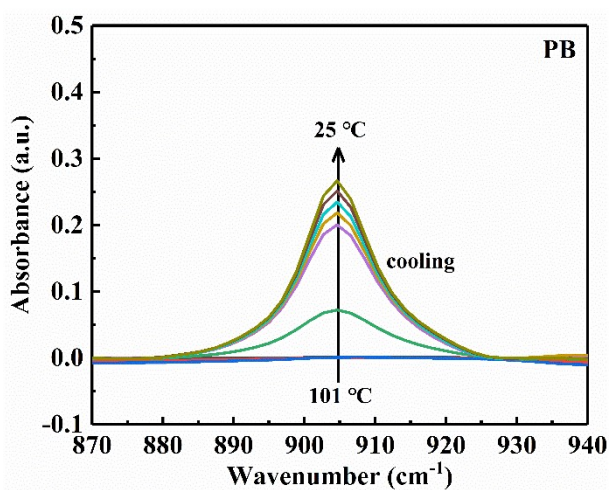
Figure S1. In-situ FTIR spectra of PB during cooling process with 10 °C/min.
