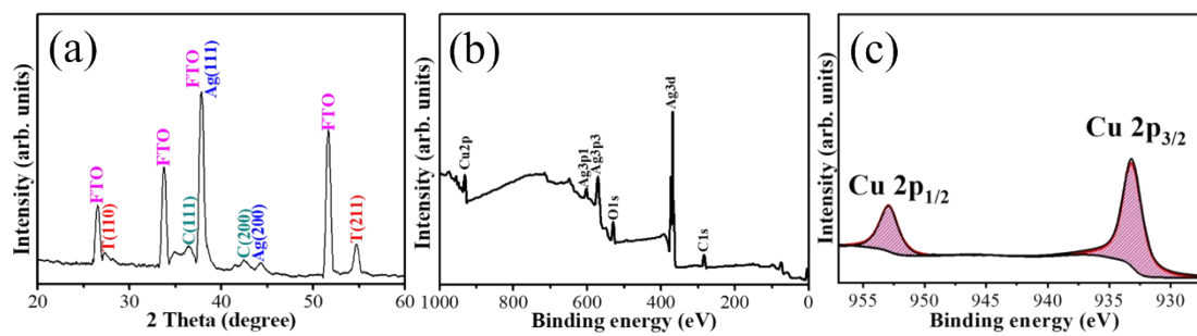
Fig. S1 Structure and chemical binding energy of the CTA 100 after five consecutive photodergadation cycles. (a) XRD pattern. (b) XPS survey scan spectrum. (c) XPS Cu 2p spectrum.
