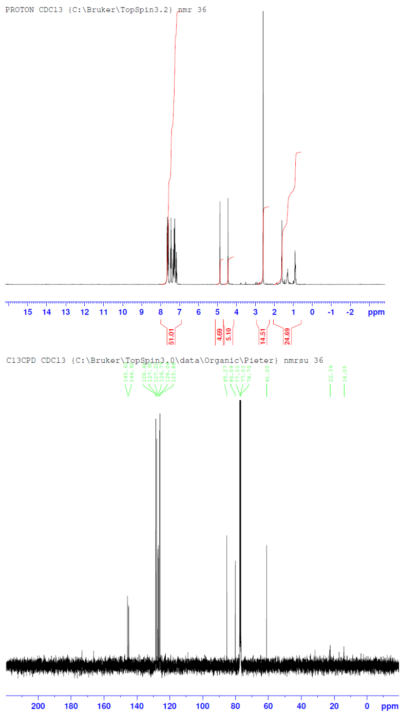
Fig. S1 1 H- (top) and 13 C- (bottom) NMR spectra for H2.
