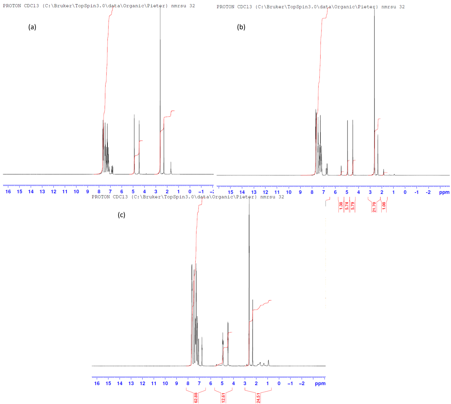
Fig. S2 ^1\text{H} -NMR spectra for (a) 2(\text{H}_2)\cdot 2\text{Cr} , (b) 2(\text{H}_2)\cdot 3\text{Cr} and (c) 2(\text{H}_2)\cdot 4\text{Cr} .
