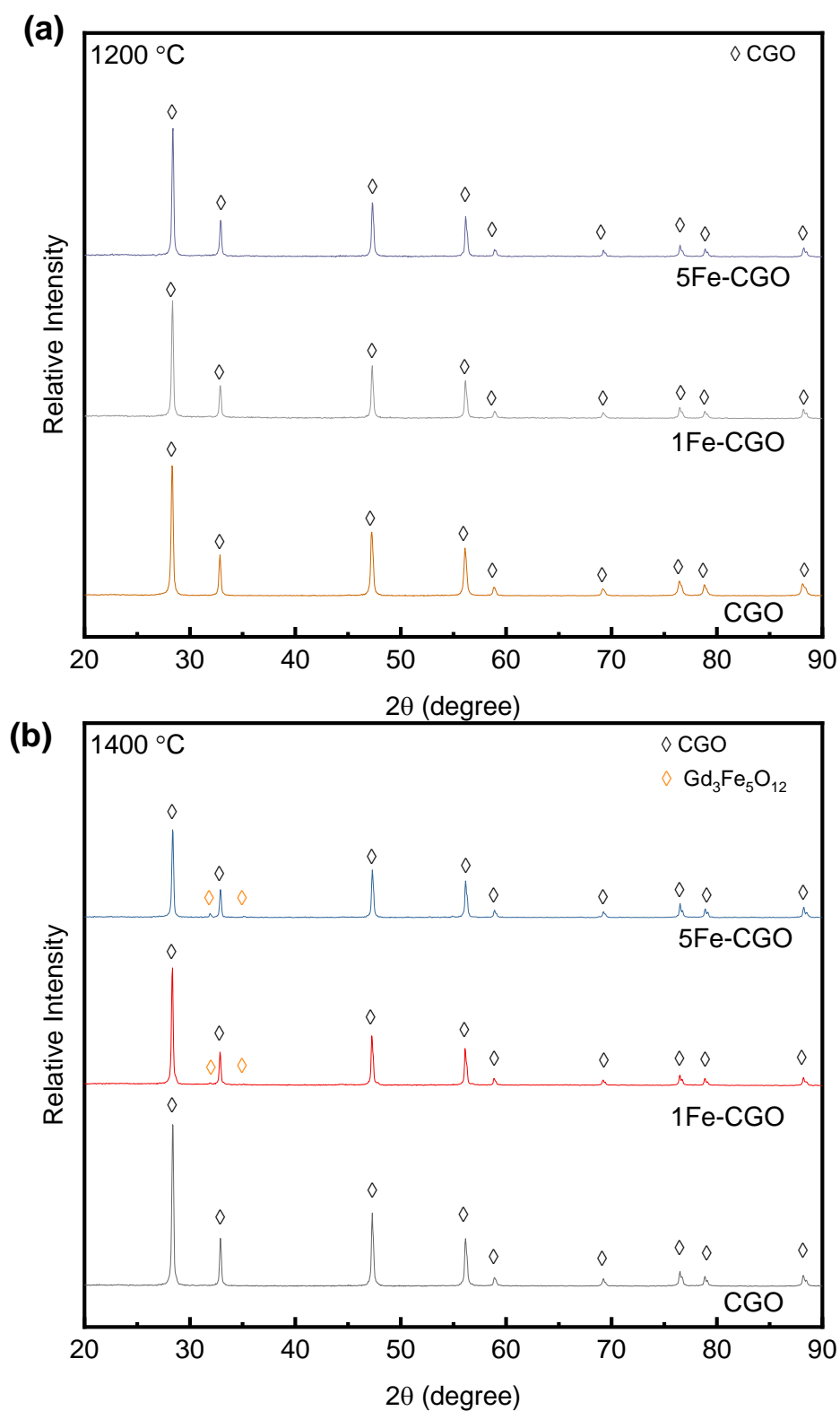
Fig. S1. X-ray diffraction patterns of CGO and Fe-doped CGO submitted to (a) 1200 °C and (b) 1400 °C.
