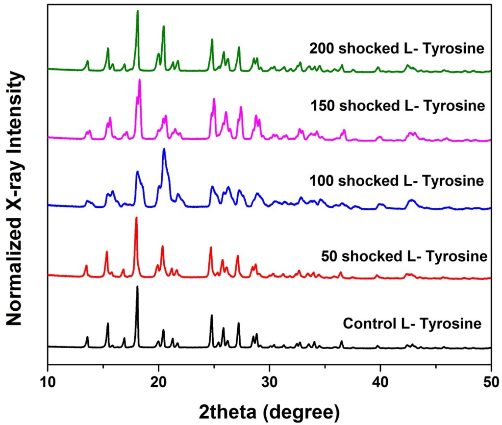
Fig.S5 XRD pattern of the control and shocked L-Tyrosine
