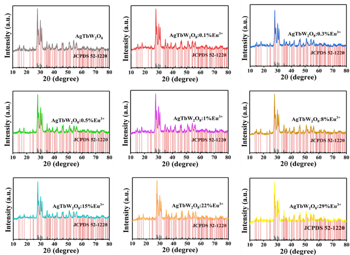
Fig. S1 XRD patterns of \text{AgTbW}_2\text{O}_8 and \text{AgTbW}_2\text{O}_8:x\%\text{Eu}^{3+} ( x = 0.1, 0.3, 0.5, 1, 8, 15, 22, 29 ).
