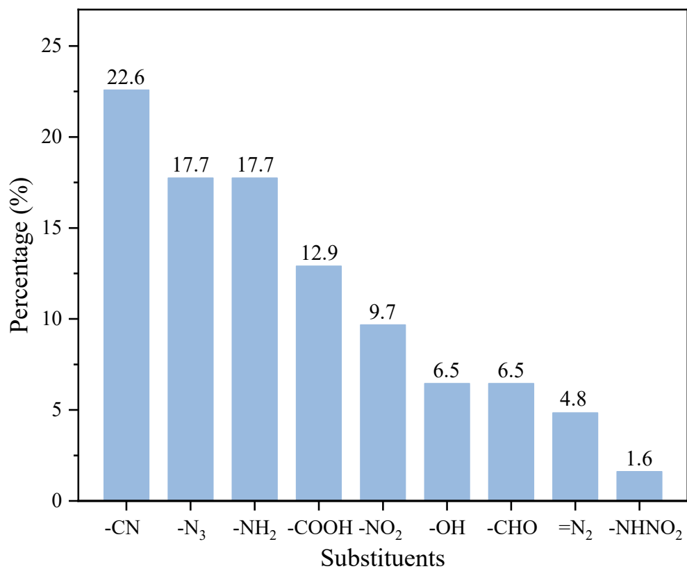
Fig. S1. Distribution of substituents of highly planar molecules with planarity of 0-0.005 Å.
