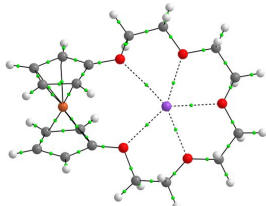
2_{\text{Fe}}^+(\text{a}) \cdots \text{Na}^+
