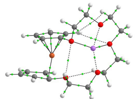
2_{\text{Fe}}(\text{a}) \cdots \text{Li}^+
