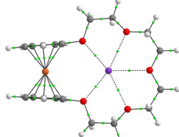
2_{\text{Fe}}(\text{a}) \cdots \text{K}^+
