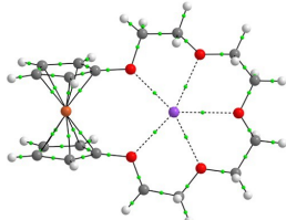
2_{\text{Fe}}(\text{a}) \cdots \text{Na}^+
