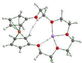
2_{\text{Fe}}^+(\text{a}) \cdots \text{Li}^+
