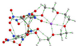
2_{\text{Fe}}(\text{c}) \cdots \text{Na}^+
