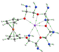
2_{\text{Fe}}^+(\text{d}) \cdots \text{Na}^+
