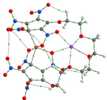
2_{\text{Fe}}^+(\text{c}) \cdots \text{Na}^+
