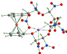
2_{\text{Fe}}(\text{e}) \cdots \text{Na}^+
