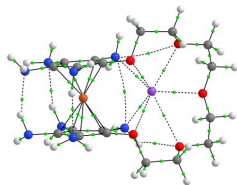
2_{\text{Fe}}(\text{b}) \cdots \text{Na}^+
