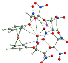
2_{\text{Fe}}^+(\text{e}) \cdots \text{Na}^+
