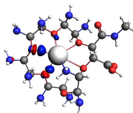
\Delta\rho_5^\sigma
