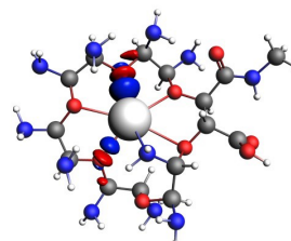
\Delta\rho_3^\sigma
