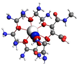
\Delta\rho_1^\sigma
