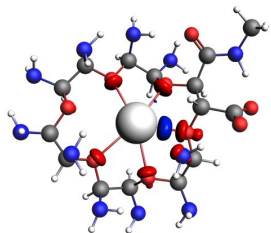
\Delta\rho_1^\sigma
