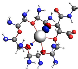
\Delta\rho_3^\sigma
