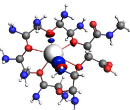
\Delta\rho_2^\sigma
