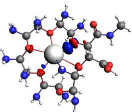
\Delta\rho_4^\sigma
