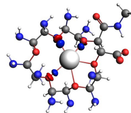
\Delta\rho_4^\sigma
