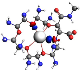
\Delta\rho_2^\sigma
