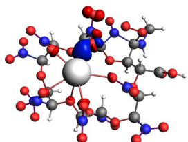
\Delta\rho_1^{\sigma \text{ and } \pi}
