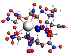
\Delta\rho_3^{\sigma \text{ and } \pi}
