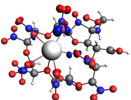
\Delta\rho_2^{\sigma \text{ and } \pi}
