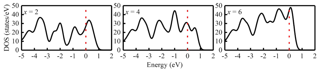
Fig. S1 Total DOS of THFS-carbon monolayer at various concentrations ( x ) of sodium.
