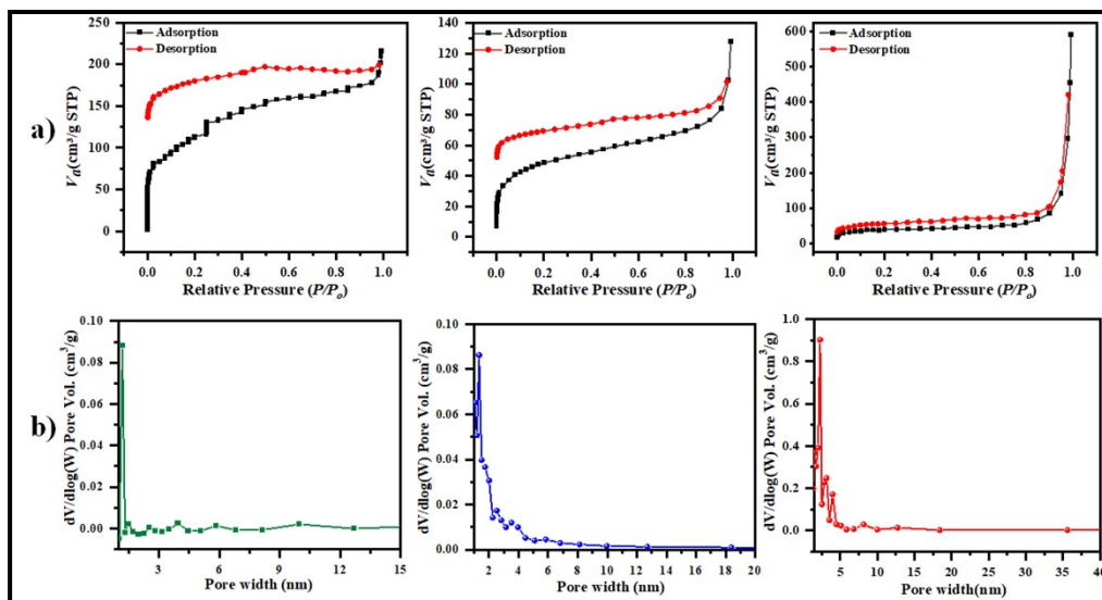
Figure S1. N_2 adsorption-desorption isotherms (a) and pore size distribution (b) of the biochar, biochar/FeS 2 , and biochar/FeS 2 /WO 3 composites.
