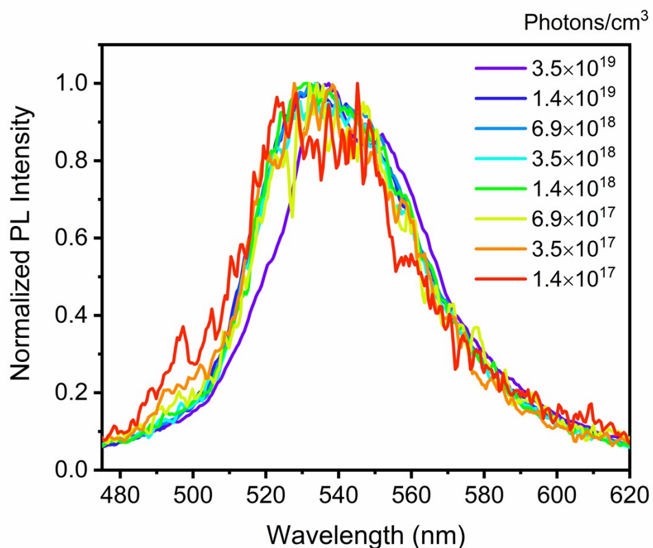
Figure S1. FAPbBr 3 PL spectra over different fluencies, confirming system stability at least for the duration of the experiment.
