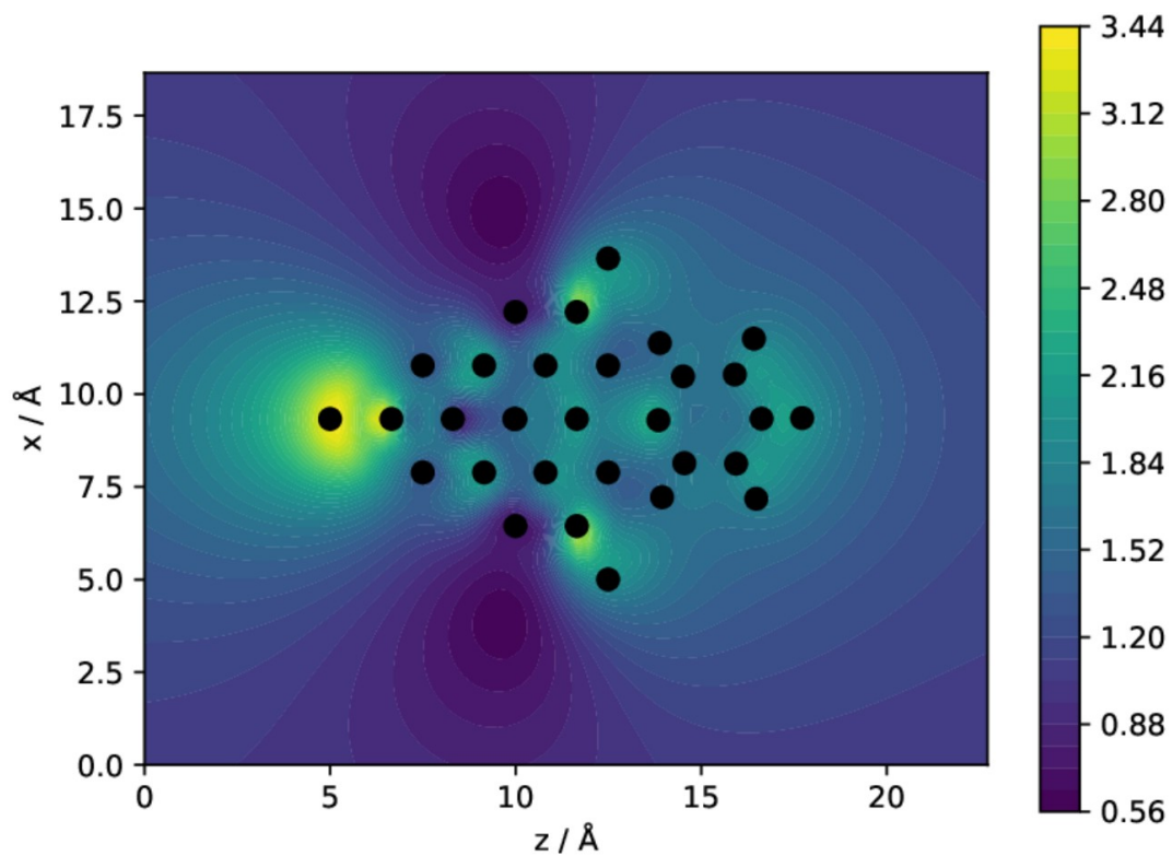
Figure S1: Electric field enhancement computed through rt-TDDFT for the pyridine@Au 20 cluster, where the pyridine molecule is situated at the center of the Au 20 surface.
