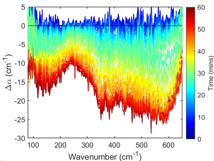
Figure S1. Example difference spectra of N1-PrP generated by the subtraction of the first spectrum from every subsequent spectrum in the measurement series up to 60 mins. The time series depicts the evolution of the LLPS as protein droplets settle on the surface of the diamond ATR crystal. The final difference spectrum from 60 mins is shown in the main text in Figure 2C.
