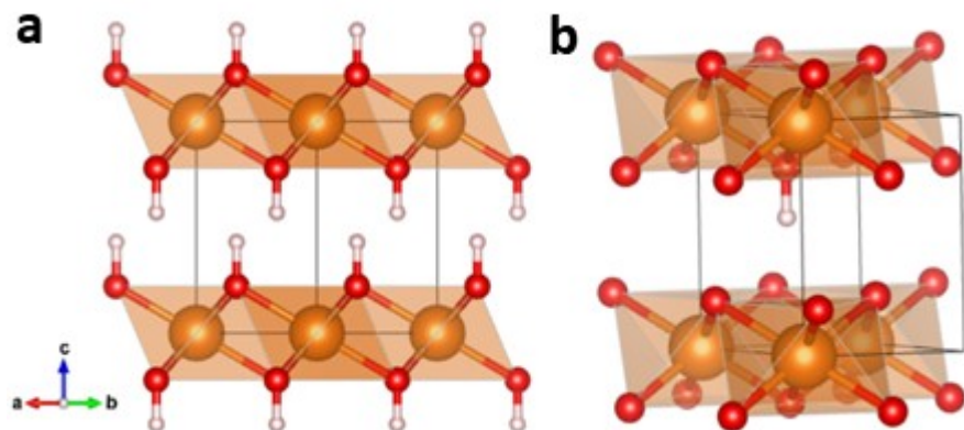
Figure S1: (a) Structure of bulk Mg(OH) 2 and (b) representation of the local environment of a OH group. Some atoms have been removed for clarity.
