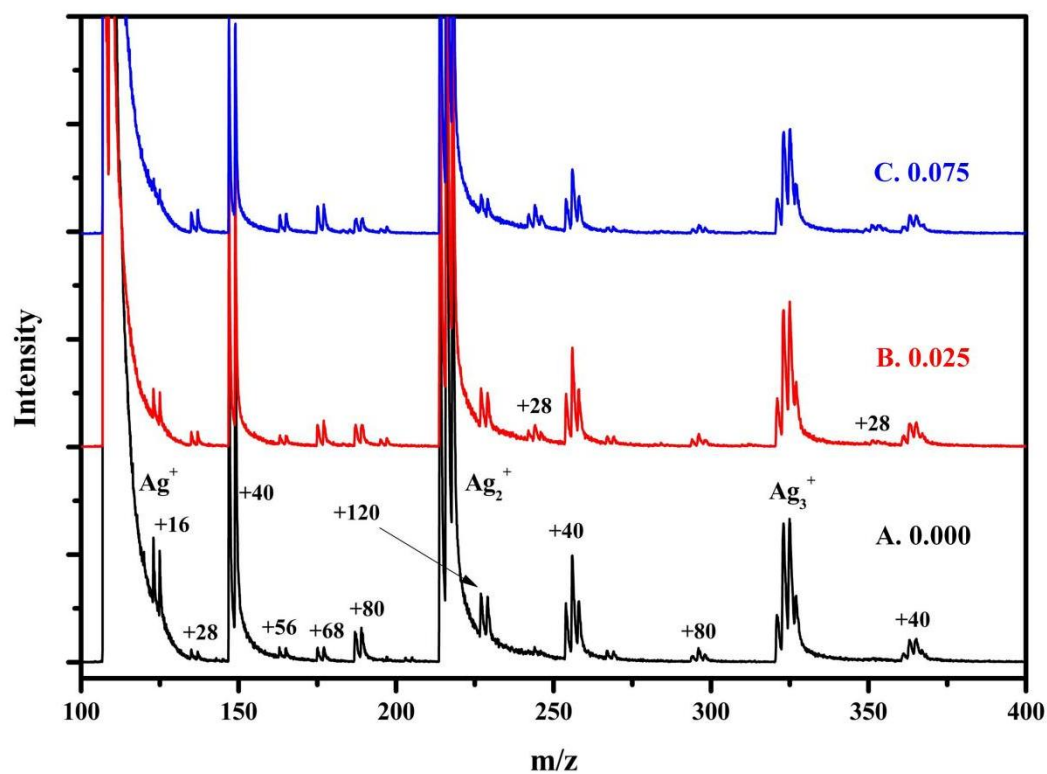
Figure S1. The mass spectra of Ag_n^+ ( n = 1-3 ) with O_2 flow of 0.000 sccm (Curve A), 0.025 sccm (Curve B) and 0.075 sccm (Curve C) at 150 K. No reaction products between Ag_n^+ ( n = 1-3 ) and O_2 were observed.
