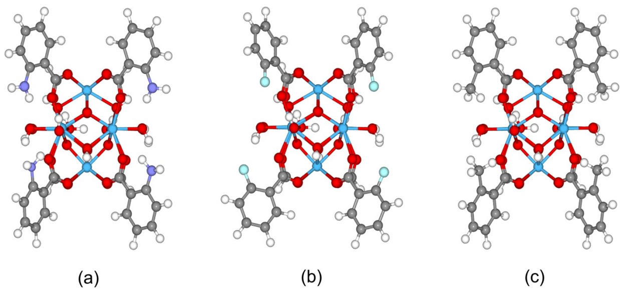
Figure S4. Cluster models of the functionalized Hf-NU-1000; (a) -NH 2 , (b) -F, and (c) -CH 3 . Hf, O, C, H, N and F are represented in blue, red, grey, white, dark blue, and green, respectively.
