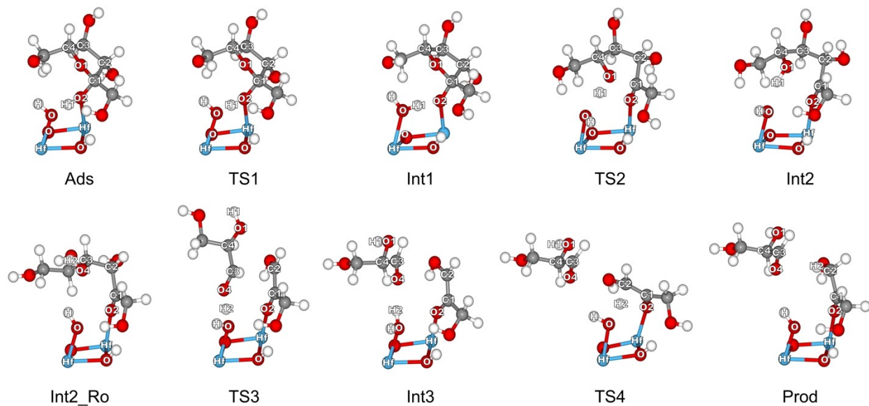
Figure S1. Optimized structures of the fructose conversion into GLA and DHA over Hf-NU-1000.
