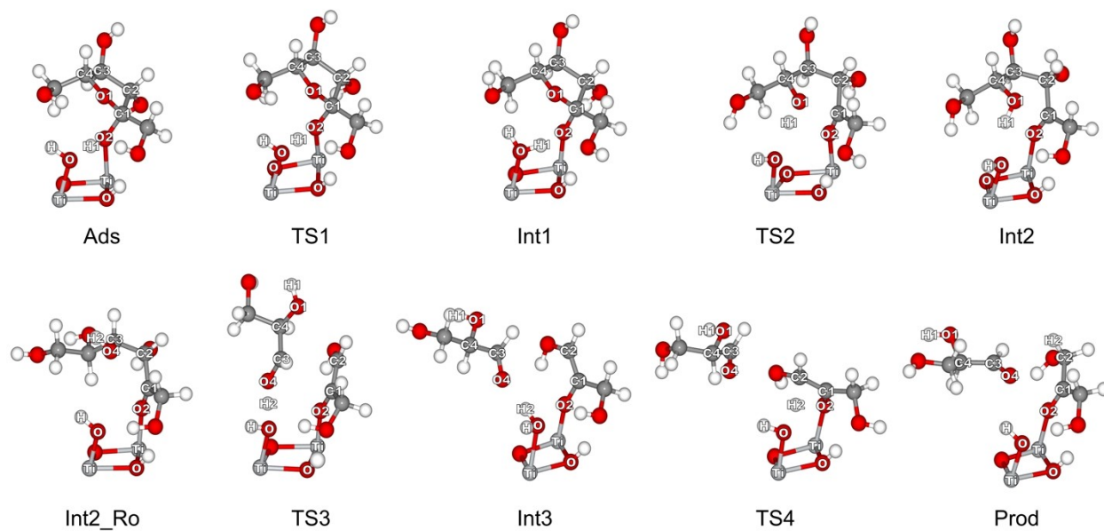
Figure S2. Optimized structures of the fructose conversion into GLA and DHA over Ti-NU-1000.
