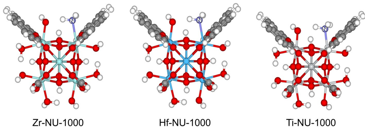
Figure S3. Optimized structures of the ammonia adsorption on NU-1000 MOFs and their binding free energies.
