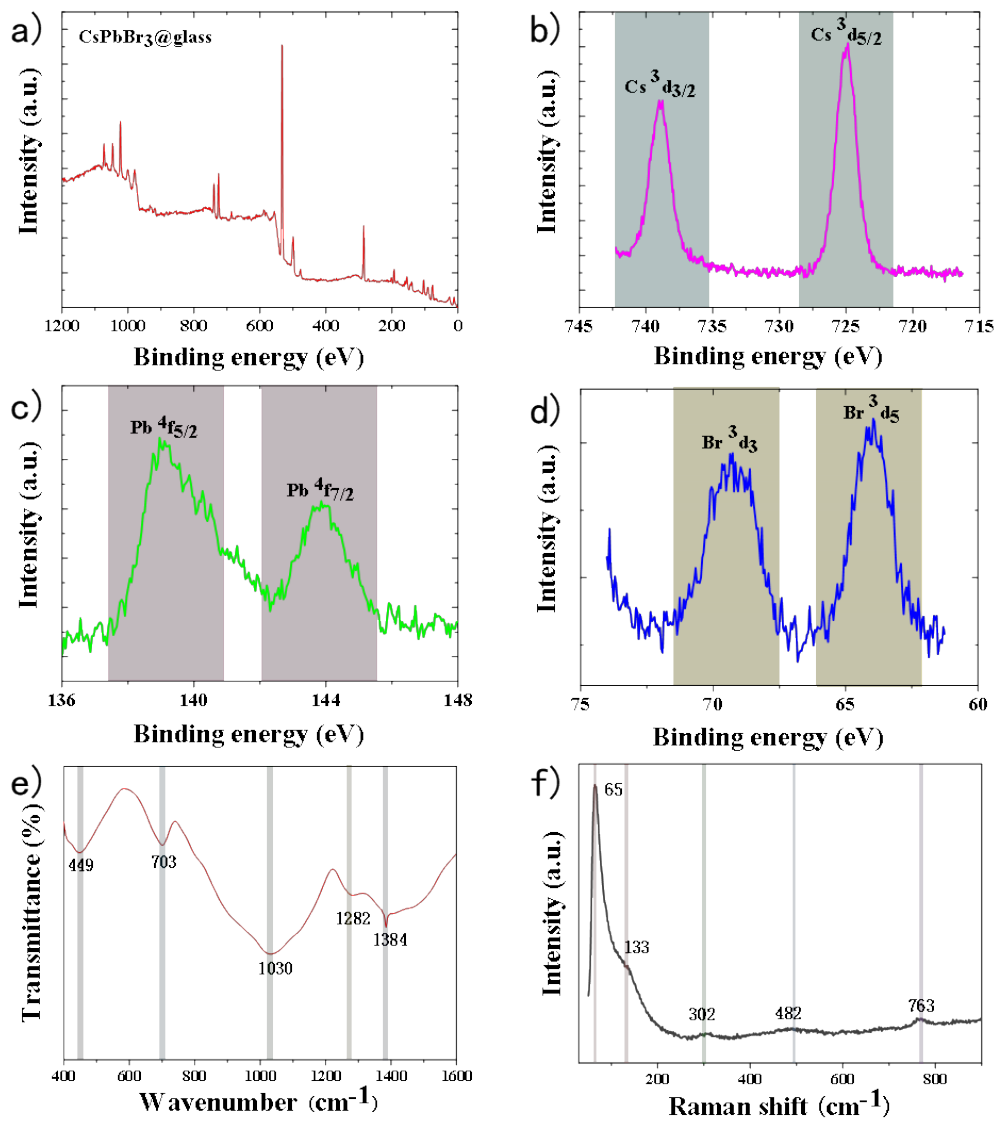
Fig. S1. a) The XPS spectrum of CsPbBr 3 @glass (a). Corresponding high-resolution spectra of Cs (b), Pb (c), Br (d). The FTIR spectrum (e) and Raman spectrum (f) of CsPbBr 3 @glass.
