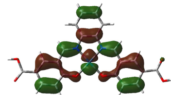
HOMO-2
