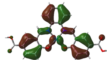
HOMO-4
