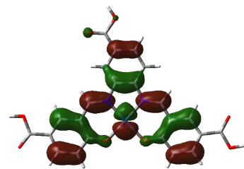
HOMO-2
