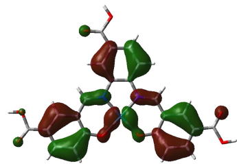
HOMO-4
