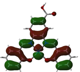
HOMO-2
