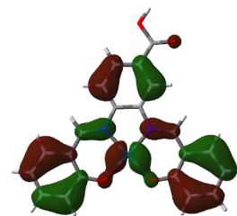
HOMO-4
