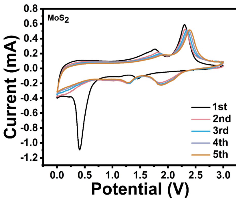
13 Fig. S2 Initial five-cycle CV curves of MoS 2 at the scan rate of 0.1 mV s -1 .
