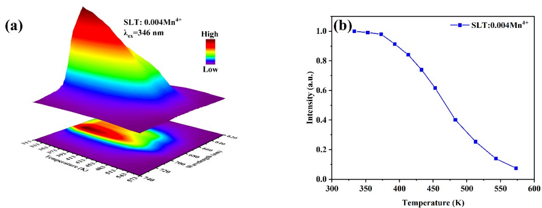
Fig. S3 (a) The PL spectra of SLT:0.004Mn 4+ at different temperature(313-573 K). (b) Integrated emission intensities of 2 E g (Mn 4+ ) of SLT:0.004Mn 4+ .
