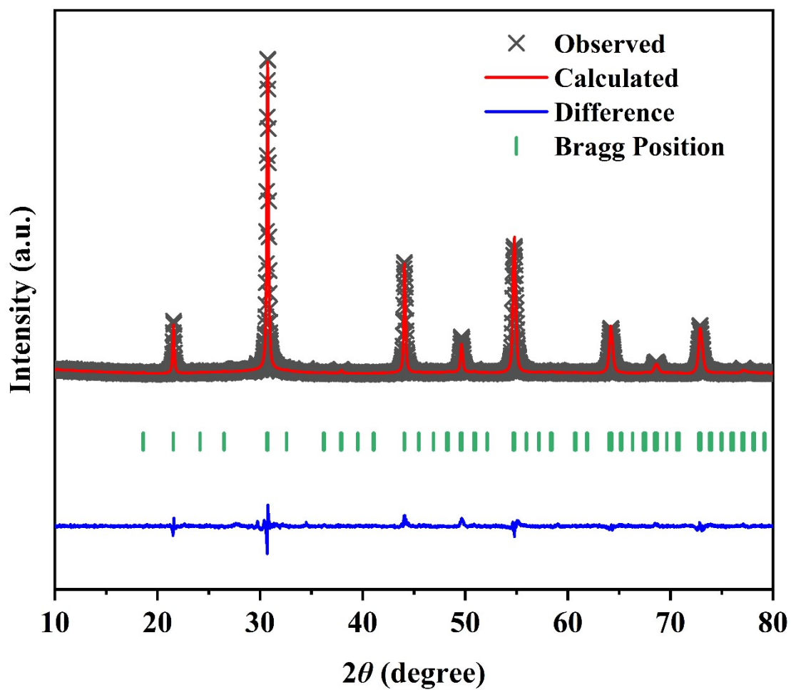
Fig. S1 Rietveld refinement result for the SLT phosphors
