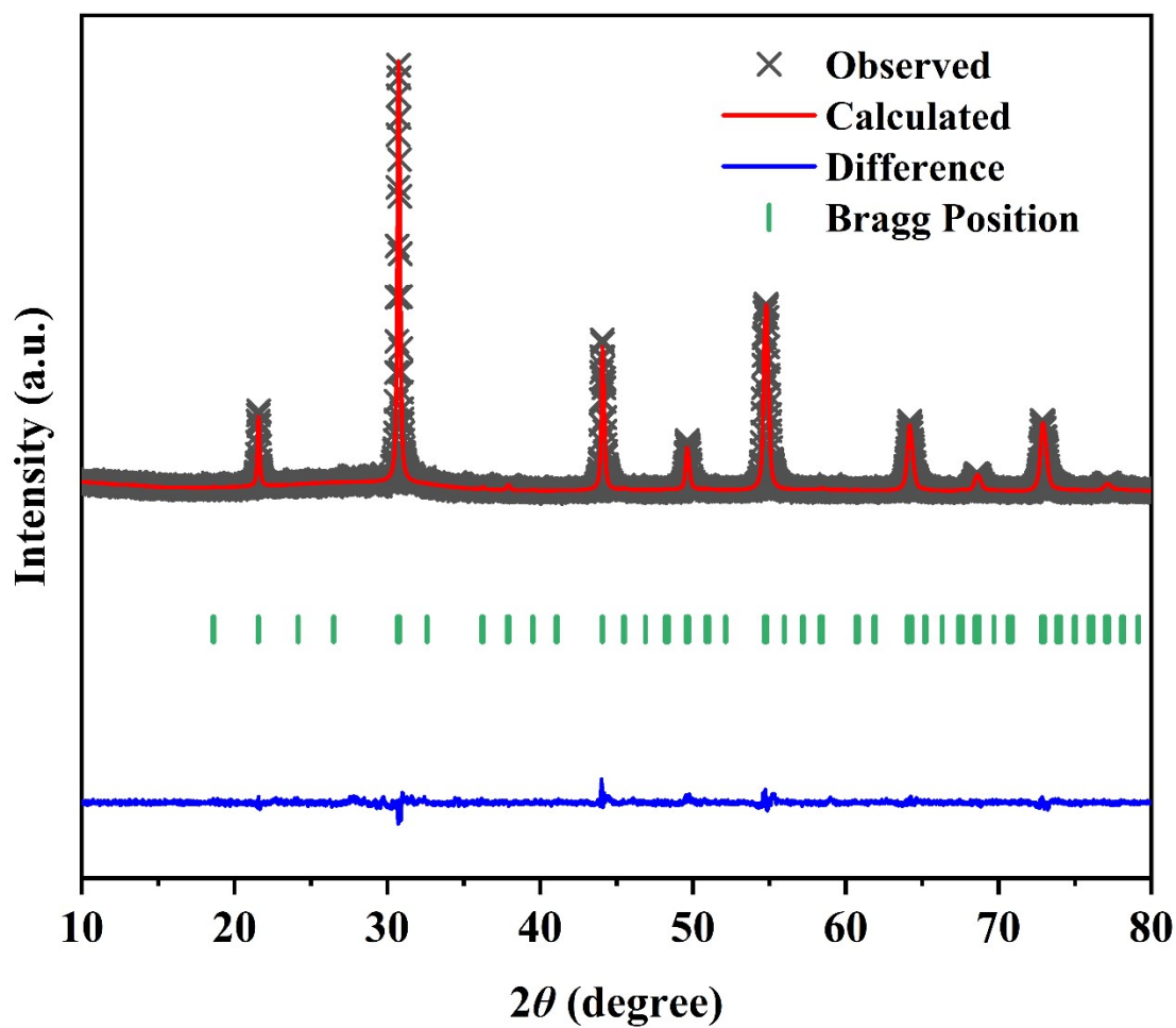
Fig. S2 Rietveld refinement result for the SLT:0.004Mn 4+ phosphors
