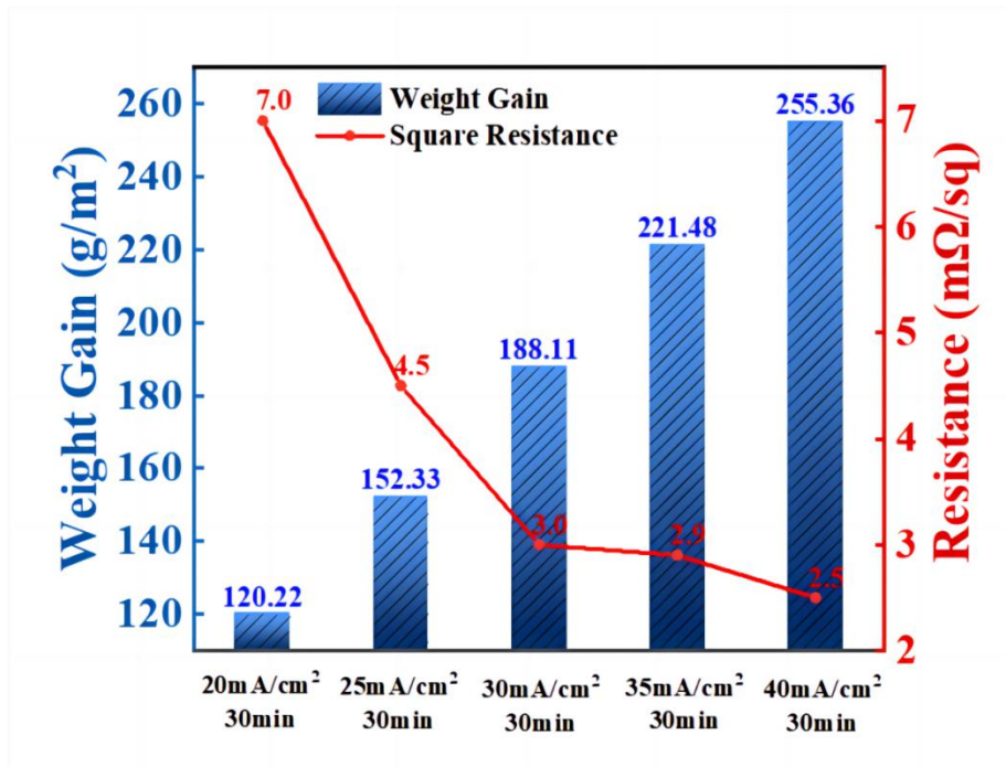
Fig. S6 Effects of current density on weight gain and electrical resistance of the Kevlar ® @Ni-P-B@Cu fabric.
