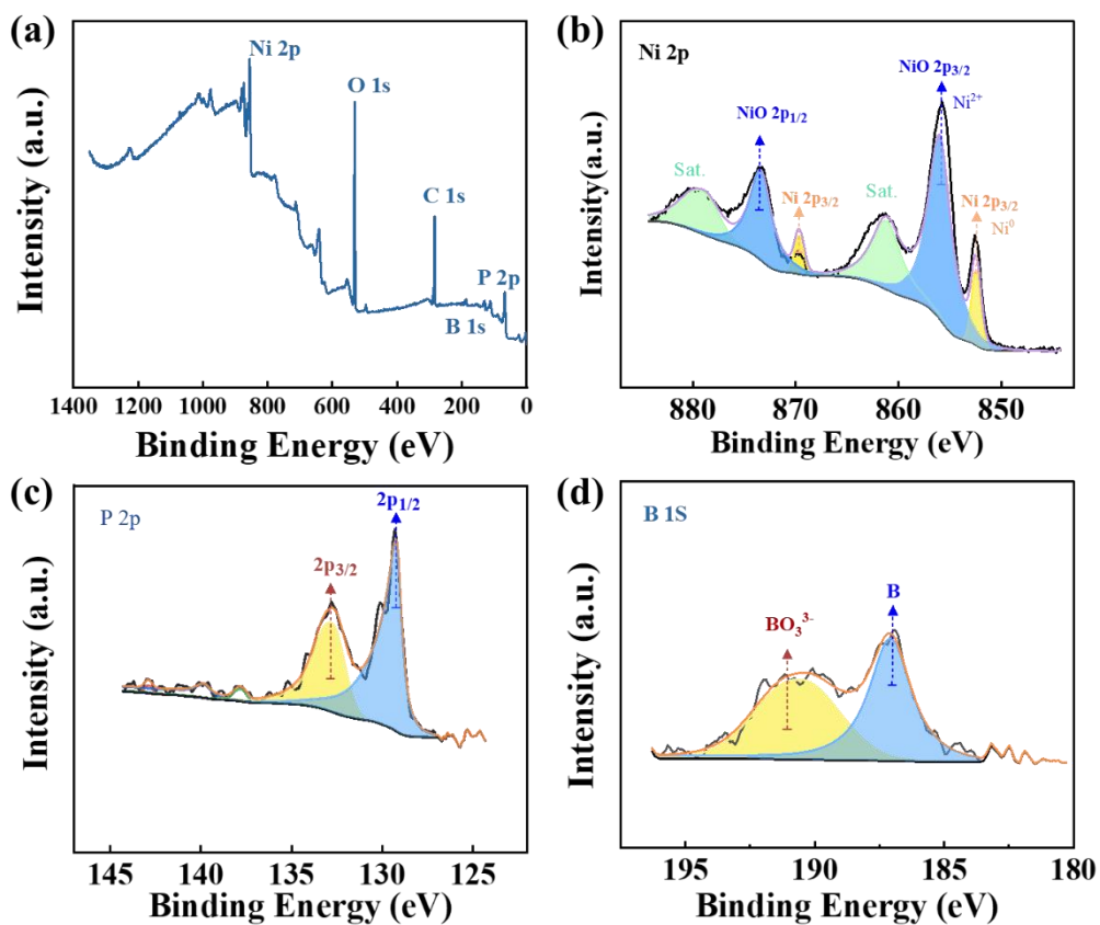
Fig. S4 XPS patterns of the Kevlar®@120-Ni-P-B fabric.
