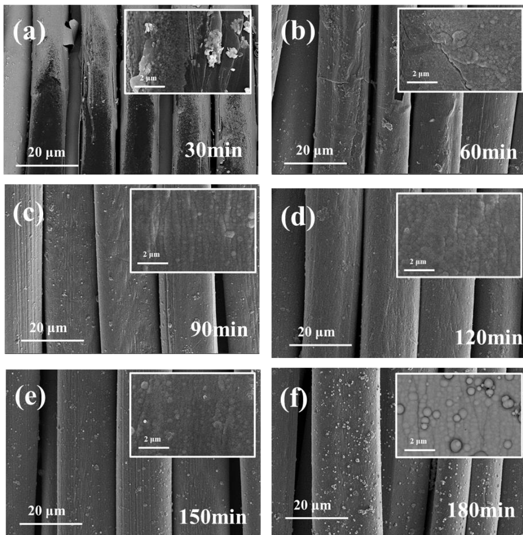
Fig. S3 SEM images of the Kevlar ® @Ni-P-B fabrics at different plating times.
