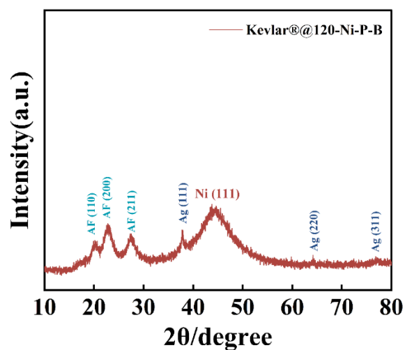
Fig. S5 XRD pattern of the Kevlar®@120-Ni-P-B fabric.
