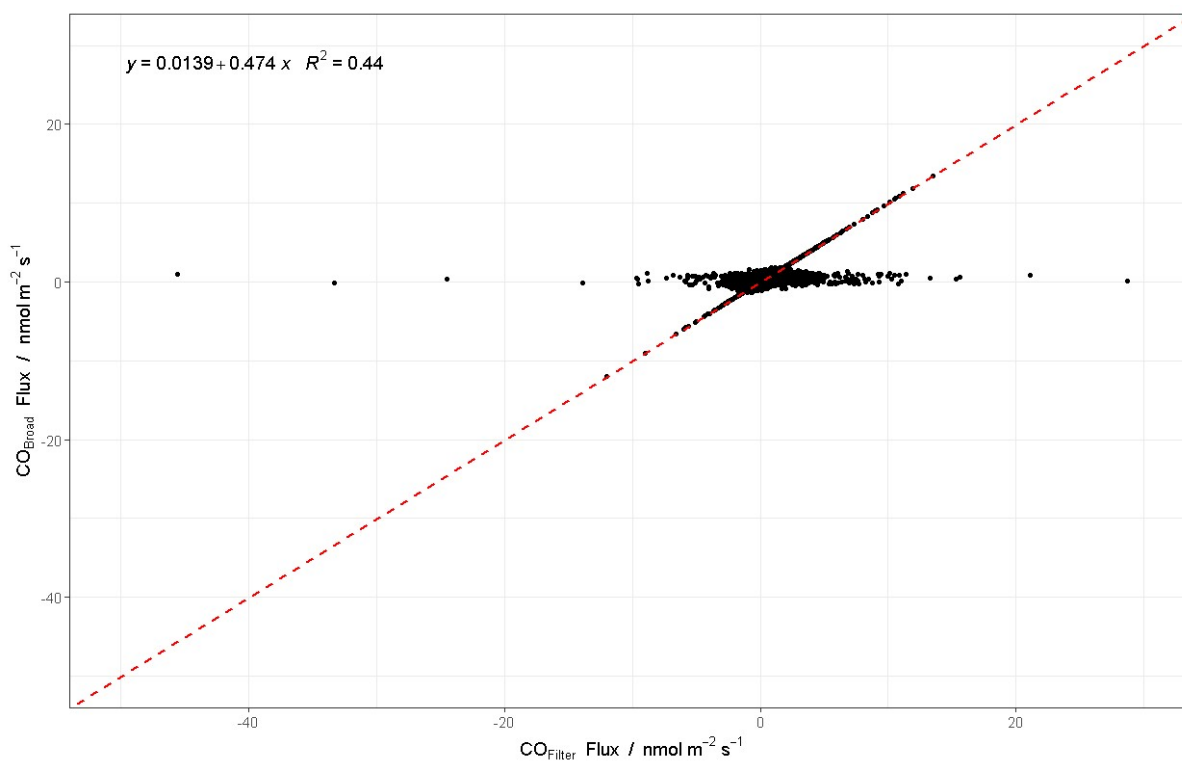
Figure S3: The relationship between modelled CO fluxes including anthropogenic sources ( \text{CO}_{\text{Broad}} ) (y-axis) and excluding anthropogenic sources \text{CO}_{\text{Filter}} (x-axis). The dashed red line represents a 1:1 relationship.
