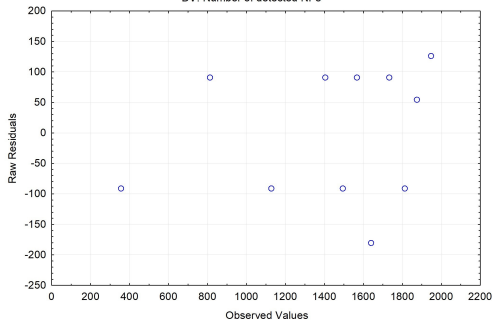
Observed vs. Residual Values
