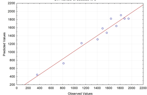
Observed vs. Predicted Values
