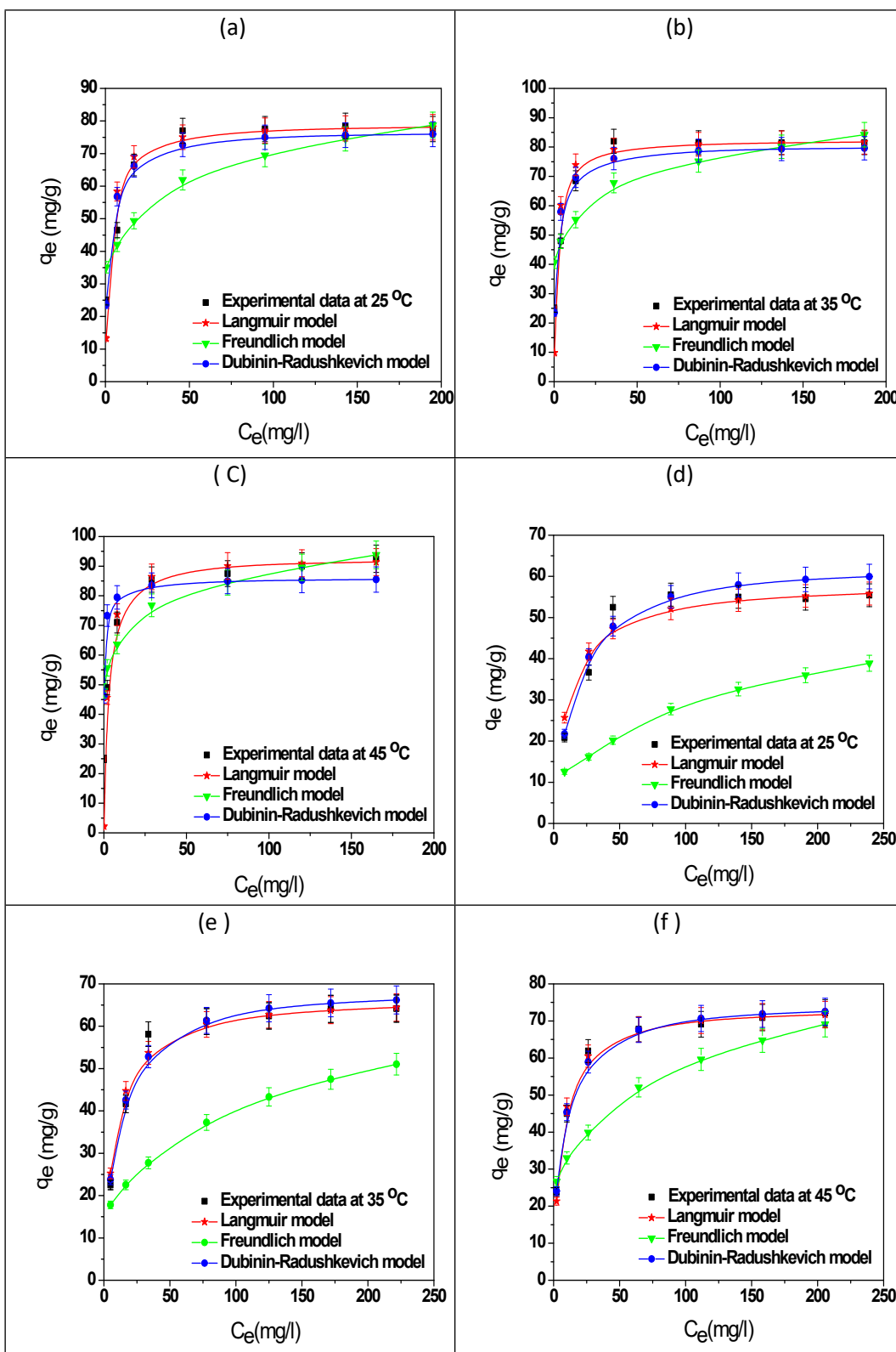
S1: Experimental sono-sorption equilibrium isotherms and non-linear models of Sr(II) and Ce(III) ions, respectively onto ST at (a,d) 25°C, (b, e) 35°C, and (c, f) 45°C.
