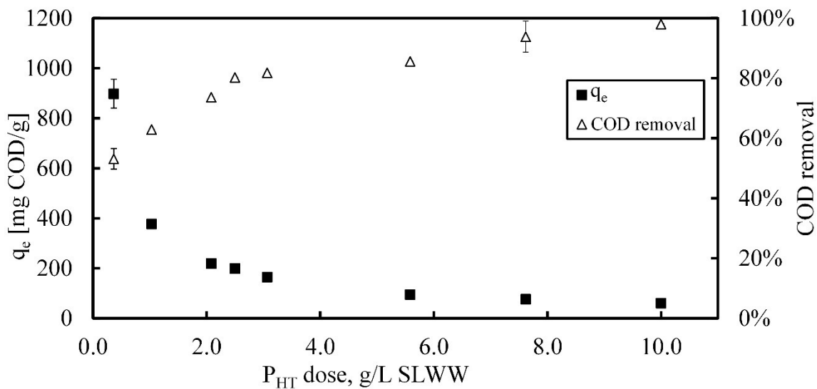
Figure S2. Effect of P_{HT} dose on the COD removal and adsorption capacity
