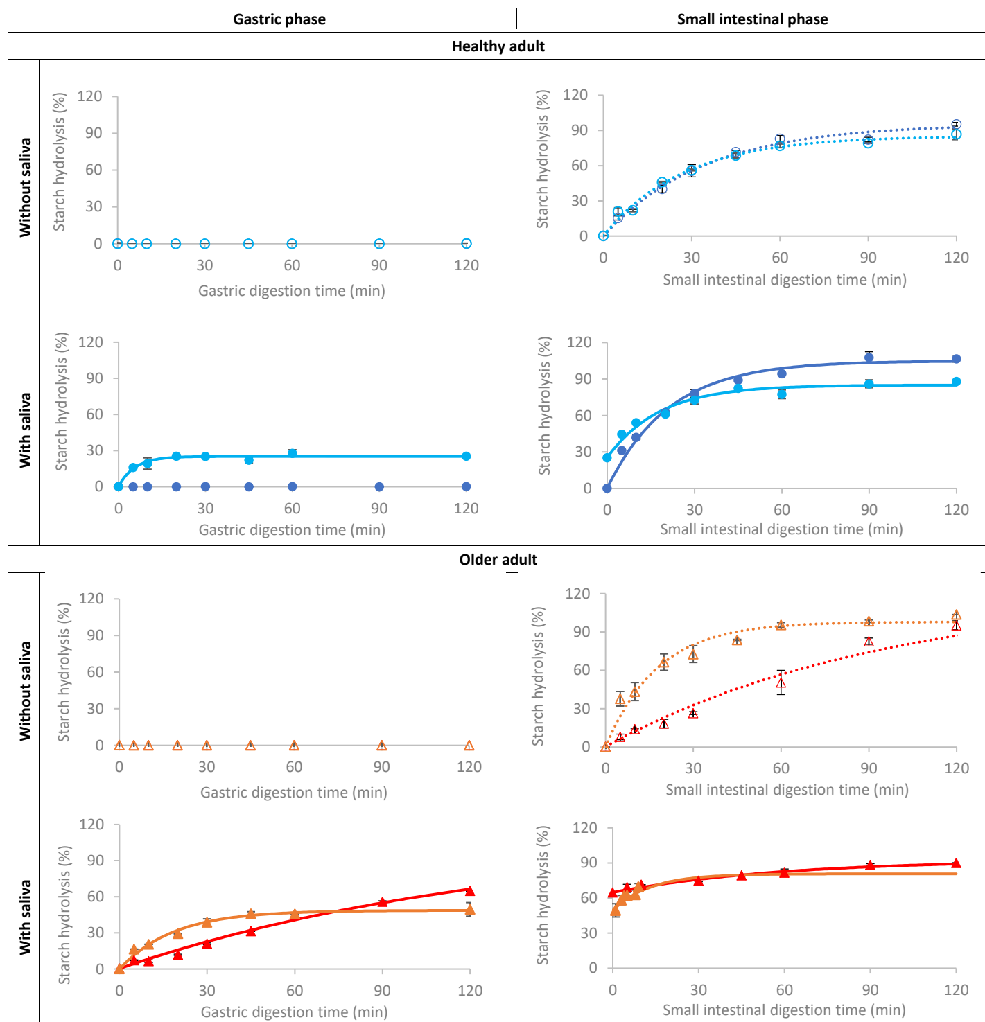
Figure C.1: Starch hydrolysis during gastric and small intestinal in vitro digestion of cooked lentils, applying models relevant for healthy adults (○/● and ◐/◑, for static and semi-dynamic models, resp.) and older adults (△/▲ and ◔/◕ for static and semi-dynamic models, resp.). Open symbols indicate simulations without addition of saliva in the oral phase, while full symbols represent simulations including saliva. The standard deviation of analytical replicates is indicated by error bars.
