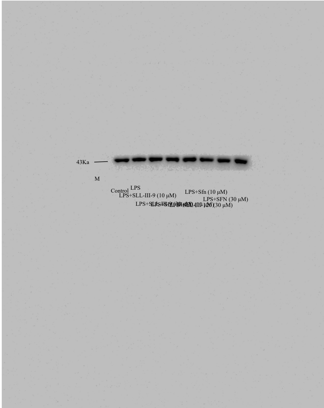
Figure 8A: β-actin
