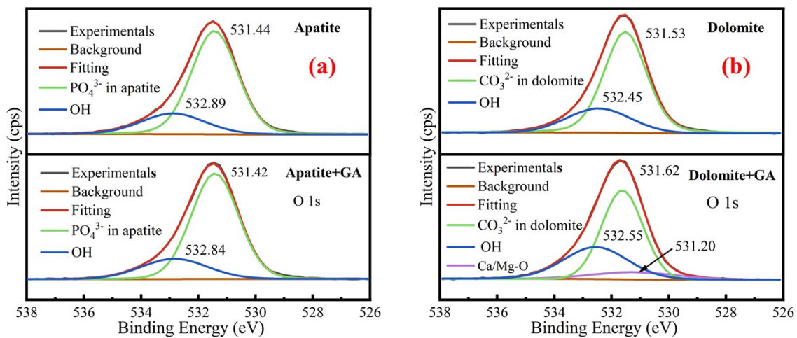
Fig. 1. XPS high-resolution spectra of O 1s on apatite (a) and dolomite (b).
