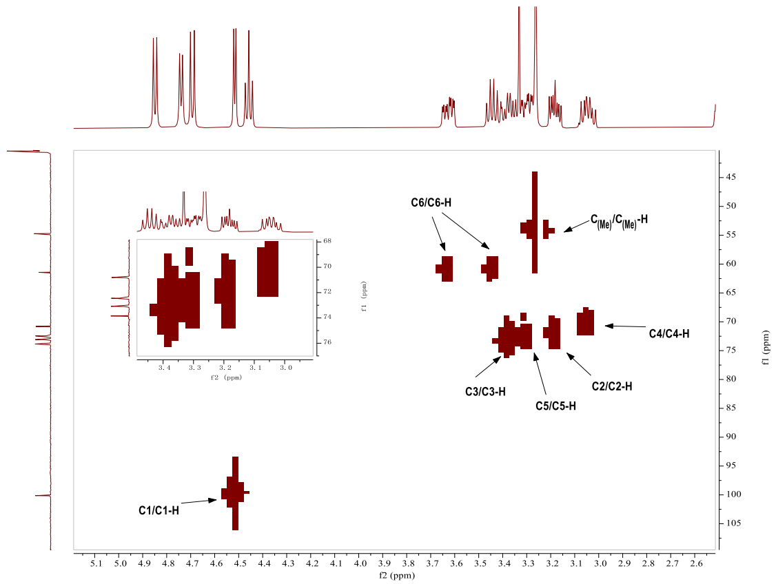
HMQC Spectra of 1a
