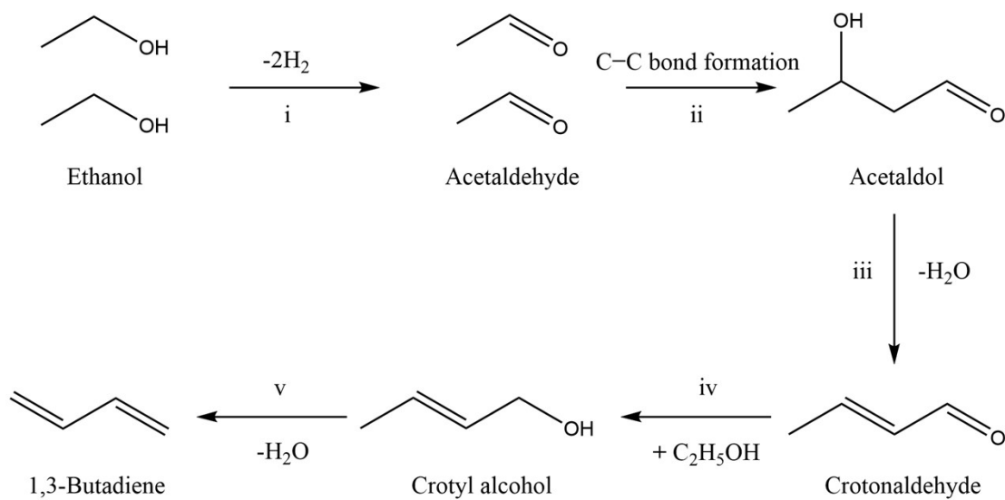
Scheme S1 mechanism for the conversion of ethanol to butadiene
