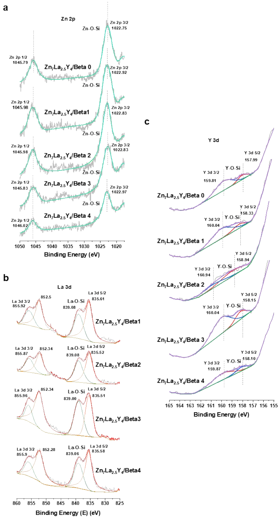
Fig. S1 the XP spectra of all ZnLaY/Beta catalysts
