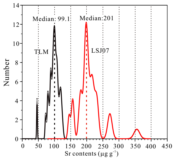
Figure S1 Sr content distributions of TLM and LSJ07
