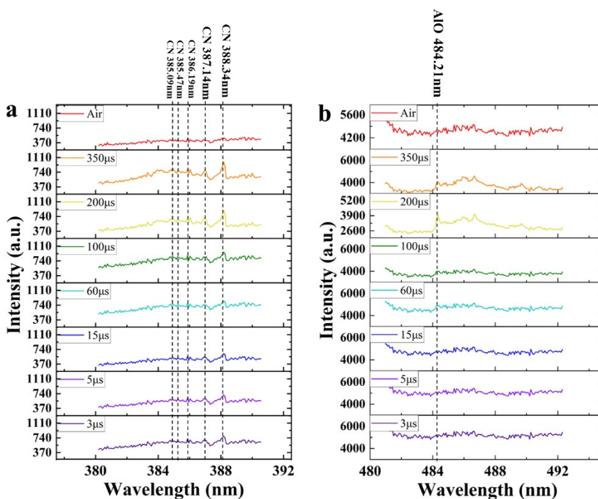
Figure S4. The comparison diagram of the background spectrum of air atmosphere and (a) CN bands and (b) AlO bands in spectra of products in air with the delay time at 3 \mu s, 5 \mu s, 15 \mu s, 60 \mu s, 100 \mu s, 200 \mu s and 350 \mu s as the distance is 7 mm.
