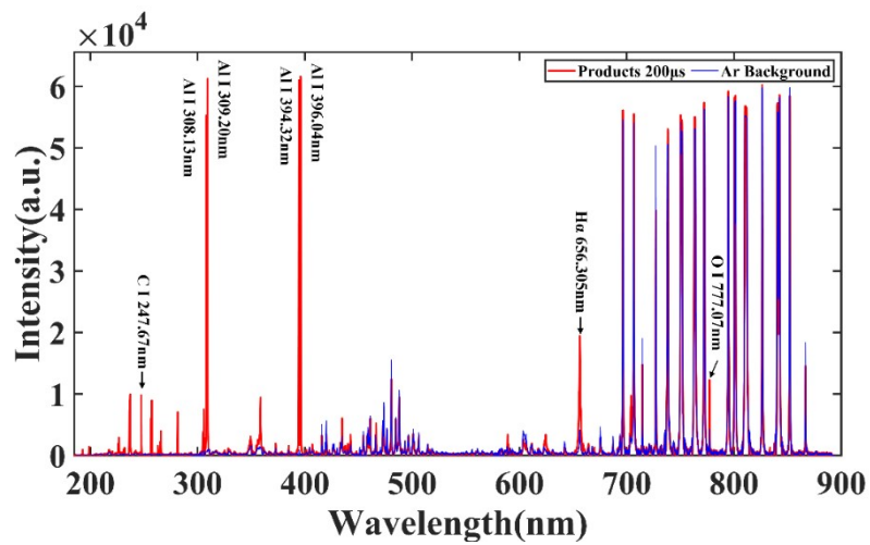
Figure S1. The comparison diagram of the background spectrum of argon atmosphere and the spectrum of products at the delay time of 200 \mu\text{s} as the distance is 5 mm.
