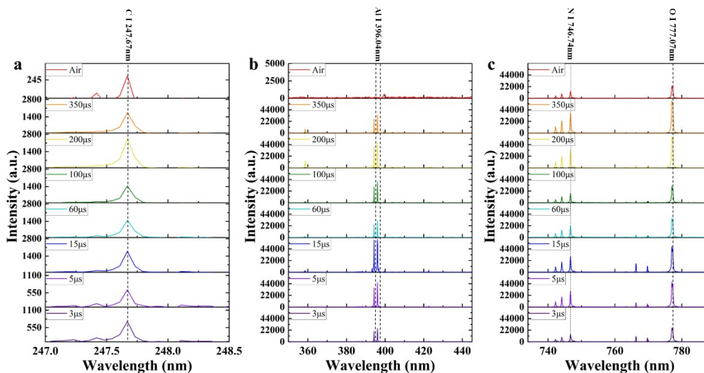
Figure S3. The comparison diagram of the background spectrum of air atmosphere and (a) C I 247.67 nm, (b) Al I 396.04 nm and (c) N I 746.74 nm, O I 777.07 nm in spectra of products in air with the delay time at 3 \mu s, 5 \mu s, 15 \mu s, 60 \mu s, 100 \mu s, 200 \mu s and 350 \mu s as the distance is 5 mm.
