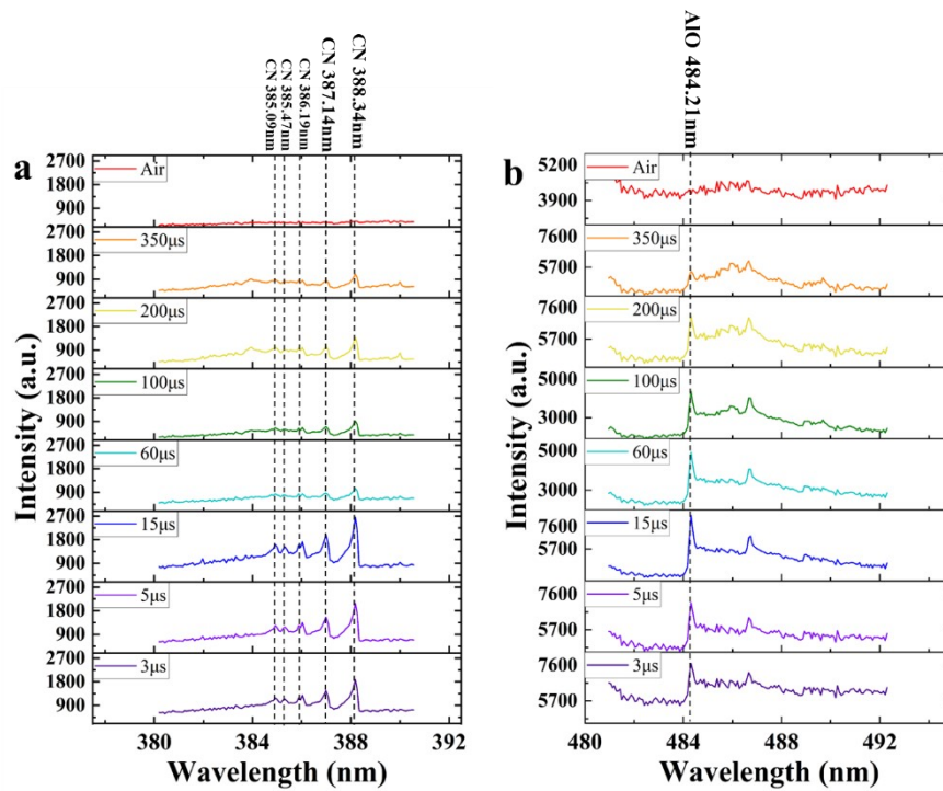
Figure S2. The comparison diagram of the background spectrum of air atmosphere and (a) CN bands and (b) AlO bands in spectra of products in air with the delay time at 3 \mu\text{s} , 5 \mu\text{s} , 15 \mu\text{s} , 60 \mu\text{s} , 100 \mu\text{s} , 200 \mu\text{s} and 350 \mu\text{s} as the distance is 5 mm.
