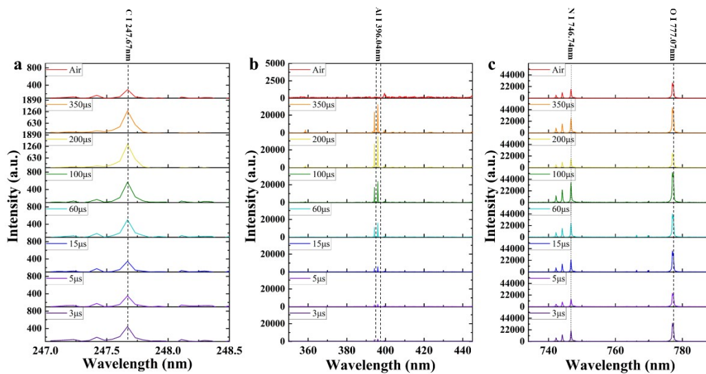
Figure S5. The comparison diagram of the background spectrum of air atmosphere and (a) C I 247.67 nm, (b) Al I 396.04 nm and (c) N I 746.74 nm, O I 777.07 nm in spectra of products in air with the delay time at 3 \mu s, 5 \mu s, 15 \mu s, 60 \mu s, 100 \mu s, 200 \mu s and 350 \mu s as the distance is 7 mm.
