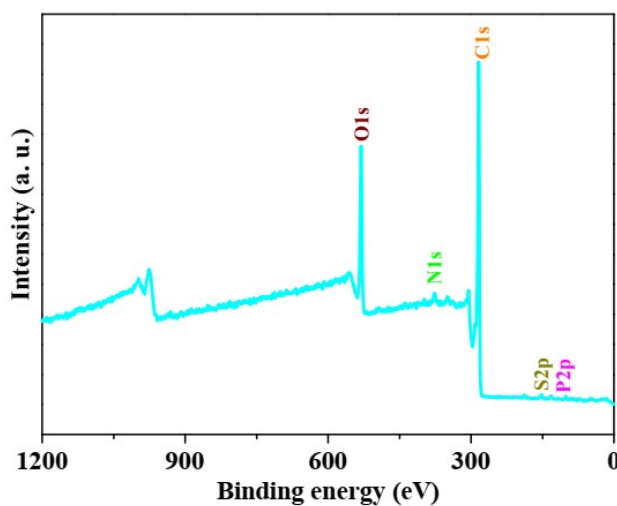
Fig. S2 XPS survey spectrum of GPAC-4
