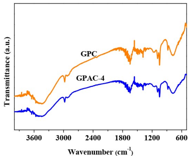
Fig. S1 FT-IR spectra of GPC and GPAC-4
